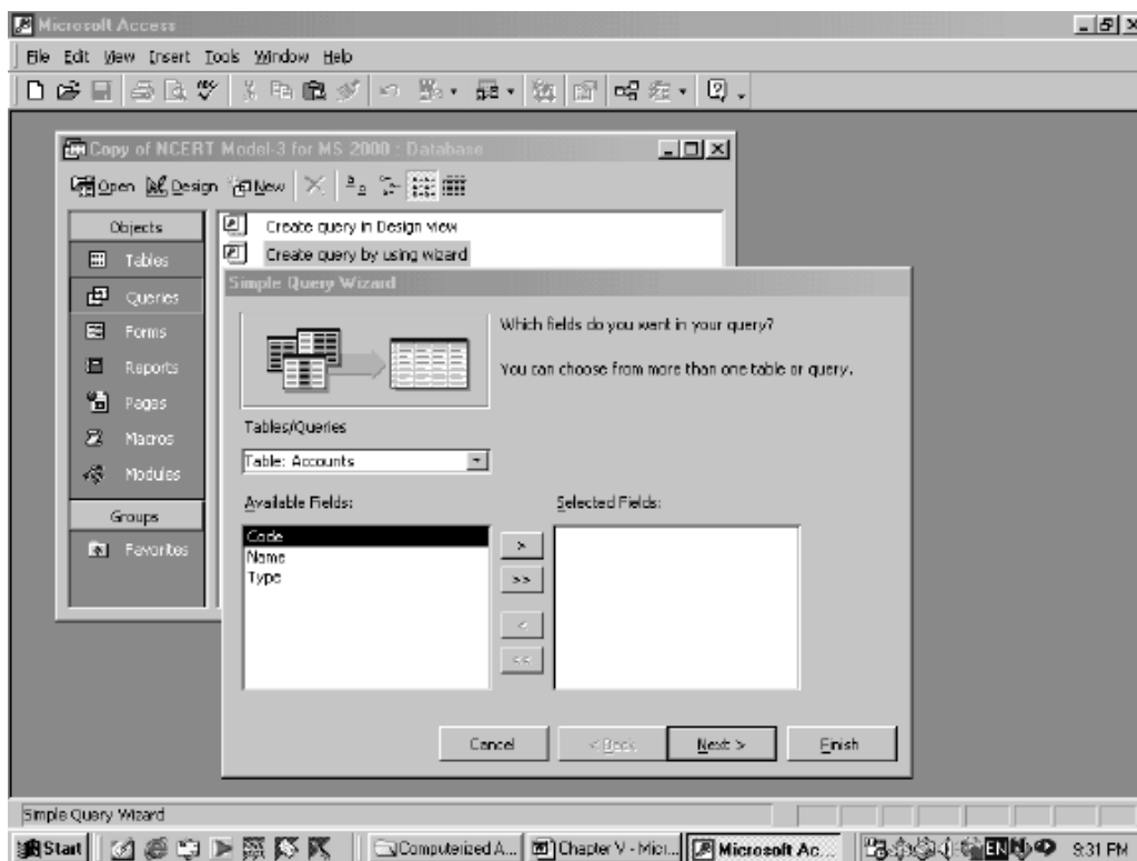
Fig. 15.6 : Window to display simple query wizard
